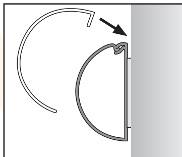
All Clip-Over accessories have grip tabs. The grip tab simply clips over the top of the length.
